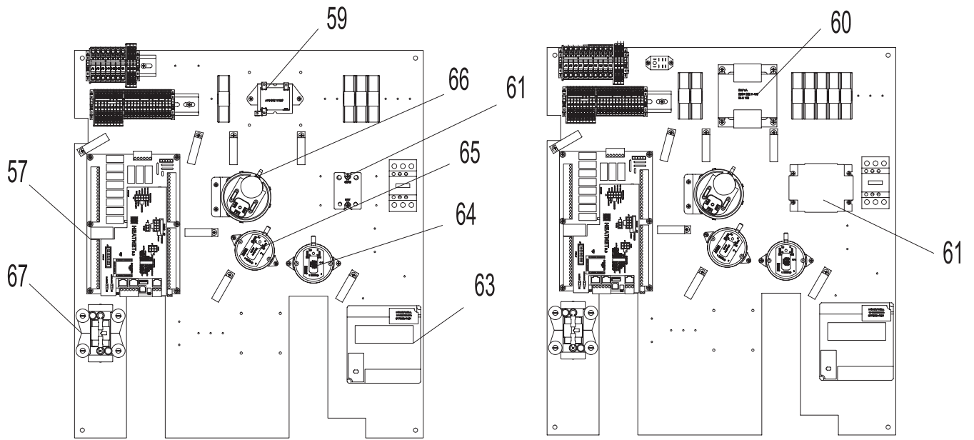
"VIEW C" (KN-6 / KN-10)
